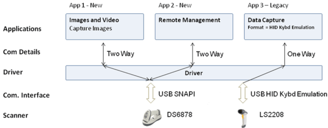
Figure 1-5 Three Applications Connected To Two Scanners
