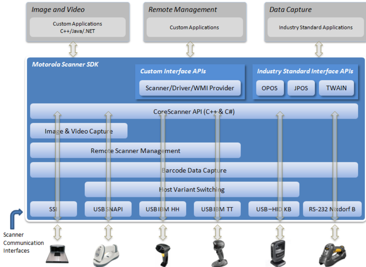
Figure 1-3 SDK Architecture
